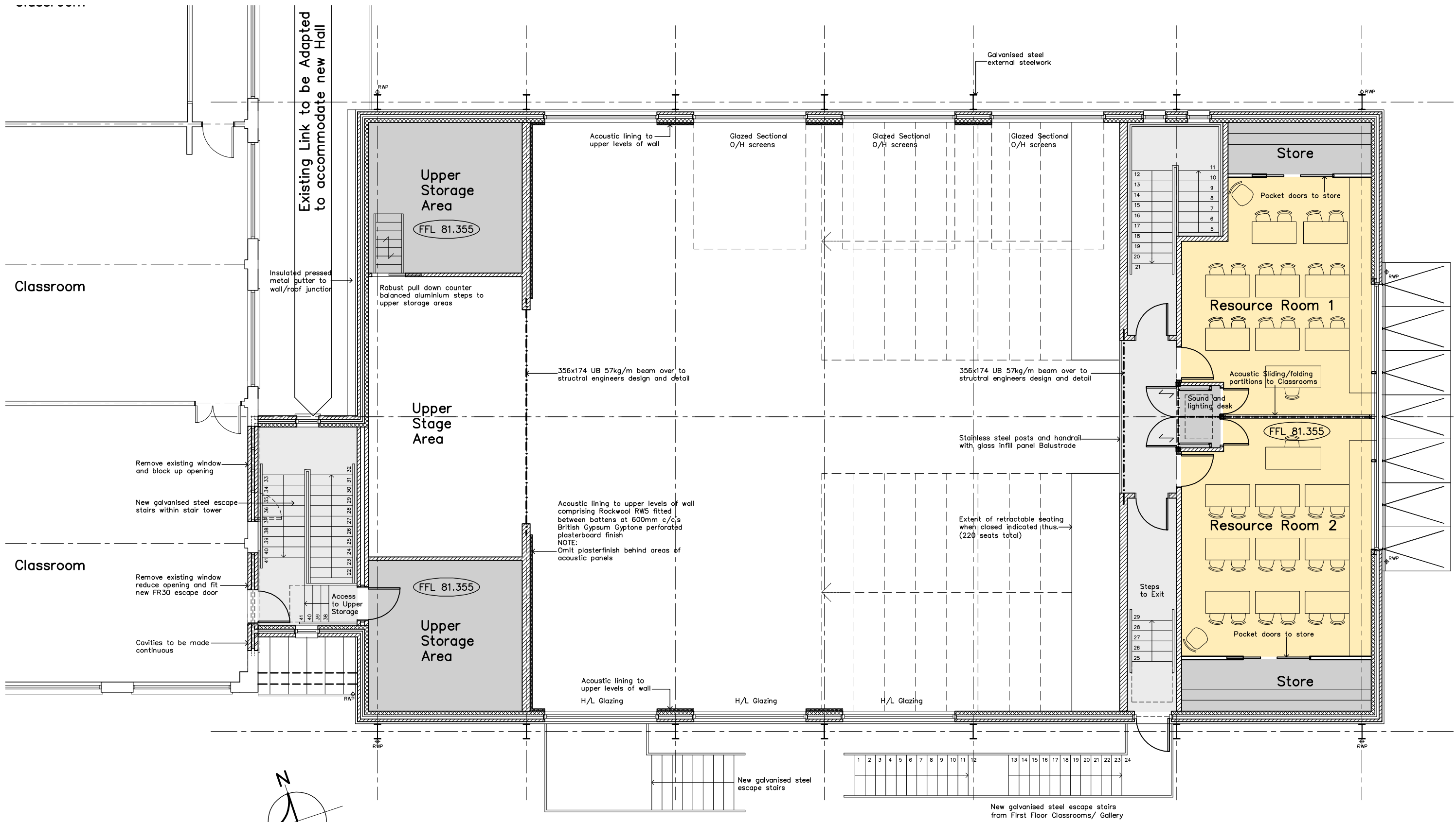
First Floor Plan scale 1:50 @ A1 (1:100 @ A3)
